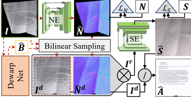
Figure 5. Proposed Refinement Network. \hat{\mathbf{B}} is the predicted backward mapping. NE is the normal estimation network and \hat{\mathbf{N}} are the predicted normals. \mathbf{I}^d and \hat{\mathbf{N}}^d are unwarped \mathbf{I} and \hat{\mathbf{N}} based on \hat{\mathbf{B}} . SE is the shading estimation network and \hat{\mathbf{S}} is the predicted shading map. \mathbf{I}^r is the concatenation ( \otimes ) of \mathbf{I}^d and \hat{\mathbf{N}}^d . \hat{\mathbf{A}} is the final shading free output and “/” represents element-wise division operator. Red dashed arrows signify the inference path.
