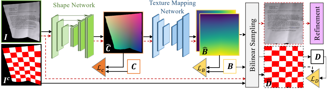
Figure 4. DewarpNet Framework. I is the input deformed document image. I^c is the I in checkerboard pattern texture. Training Flow is in black lines. The two black dashed lines refer to the predicted ( \hat{D} ) and ground-truth ( D ) unwarped reconstruction patterns. Testing flow is in red dashed lines. Triangles denote the losses (see Sec. 4.2 for details). C and B are the ground-truth for the 3D coordinates and the backward mapping respectively.
