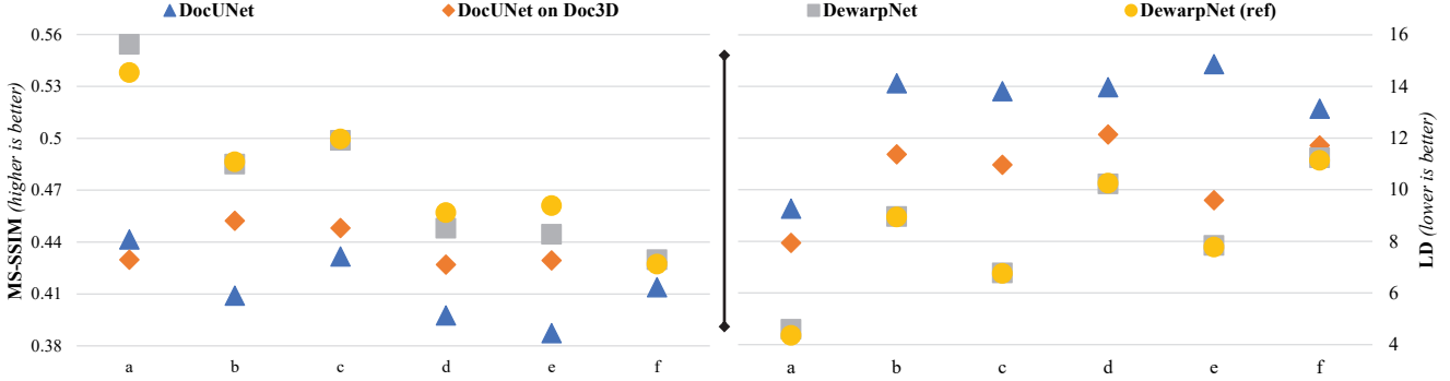
Figure 6. Comparison of different methods on deformation classes. We evaluate the results on: i) MS-SSIM ( higher is better ) and ii) LD ( lower is better ); Labels on x-axis correspond to the deformation classes (a)-(f) (as defined in Sec. 5.1).
