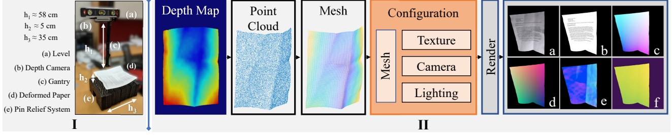
Figure 3. Data collection pipeline. I. Workstation. A leveled depth camera mounted on a gantry captures the deformed document. A pin relief system precisely controls the warping. II. Data processing. We turned the depth map into a point cloud to reconstructed a mesh. With multiple rendering configurations, we rendered (a) images, (b) albedo maps, (c) UV maps, (d) 3D coordinate maps, (e) Surface normals, (f) depth maps
