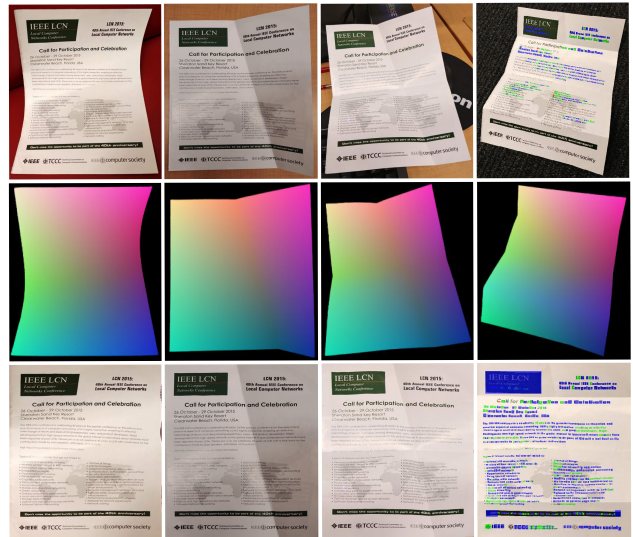
Figure 1. Document image unwarping. Top row: input images. Middle row: predicted 3D coordinate maps. Bottom row: predicted unwarped images. Columns from left to right: 1) curled, 2) one-fold, 3) two-fold, 4) multiple-fold with OCR confidence highlights in Red (low) to Blue (high).
